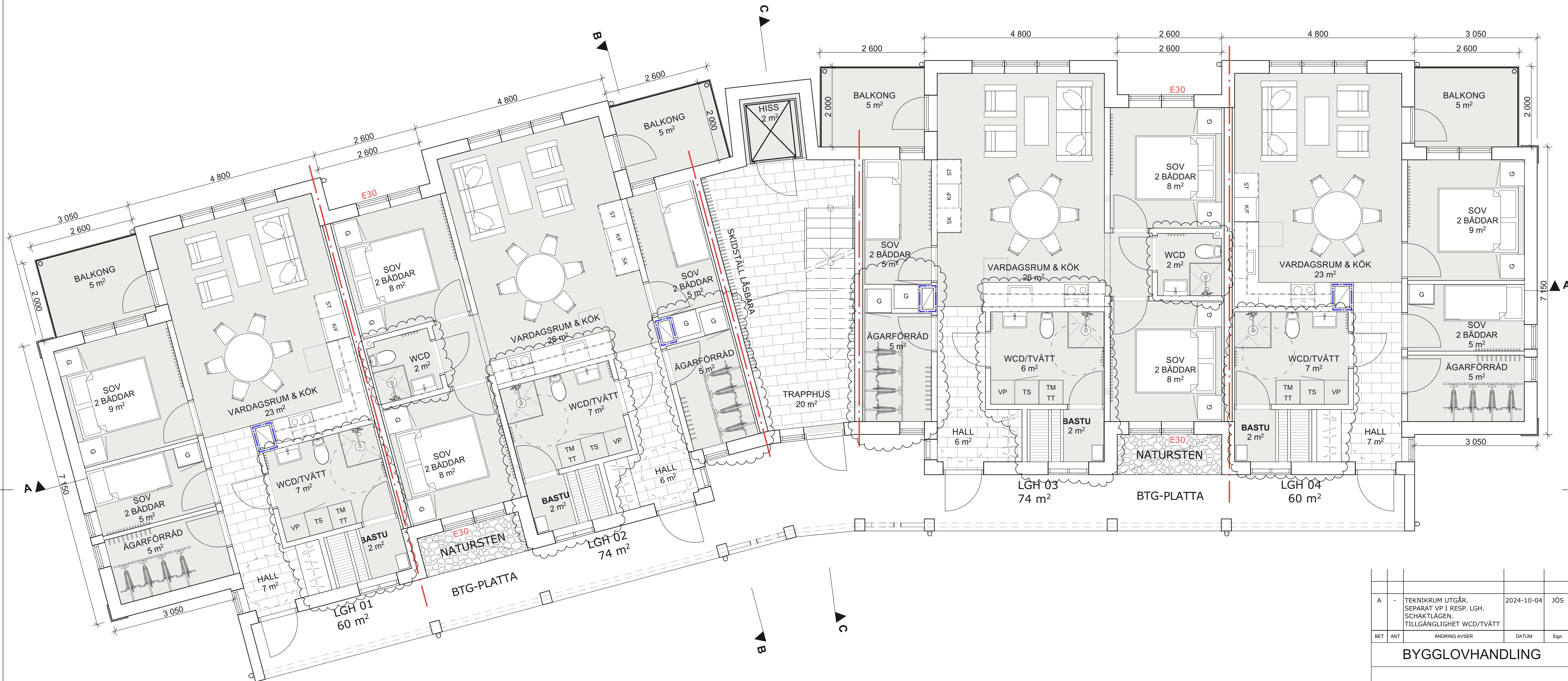
PLAN 1 - MARKPLAN
